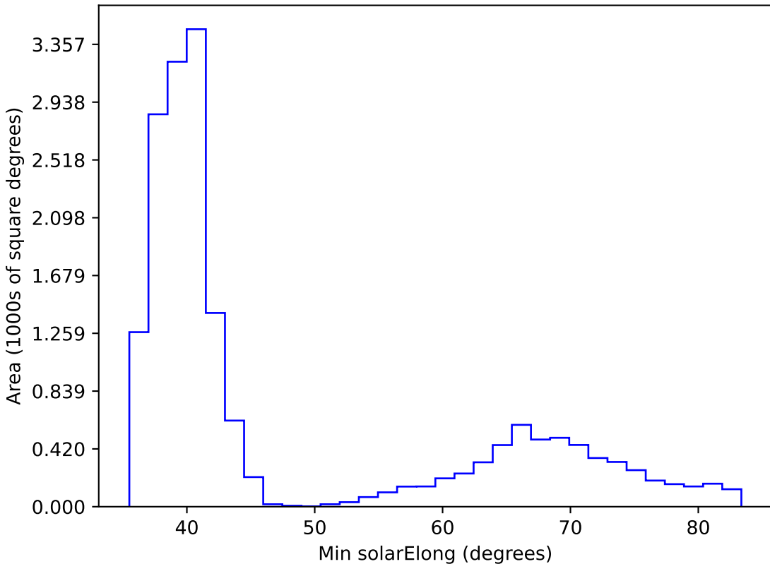
noroll_mjdp270_v3.4_10yrs WFD all bands: Min solarElong
