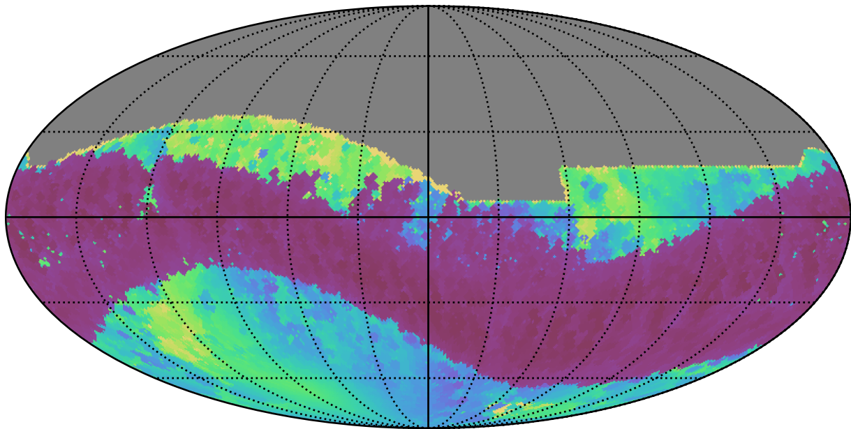
noroll_mjdp270_v3.4_10yrs All sky z band: Min solarElong
