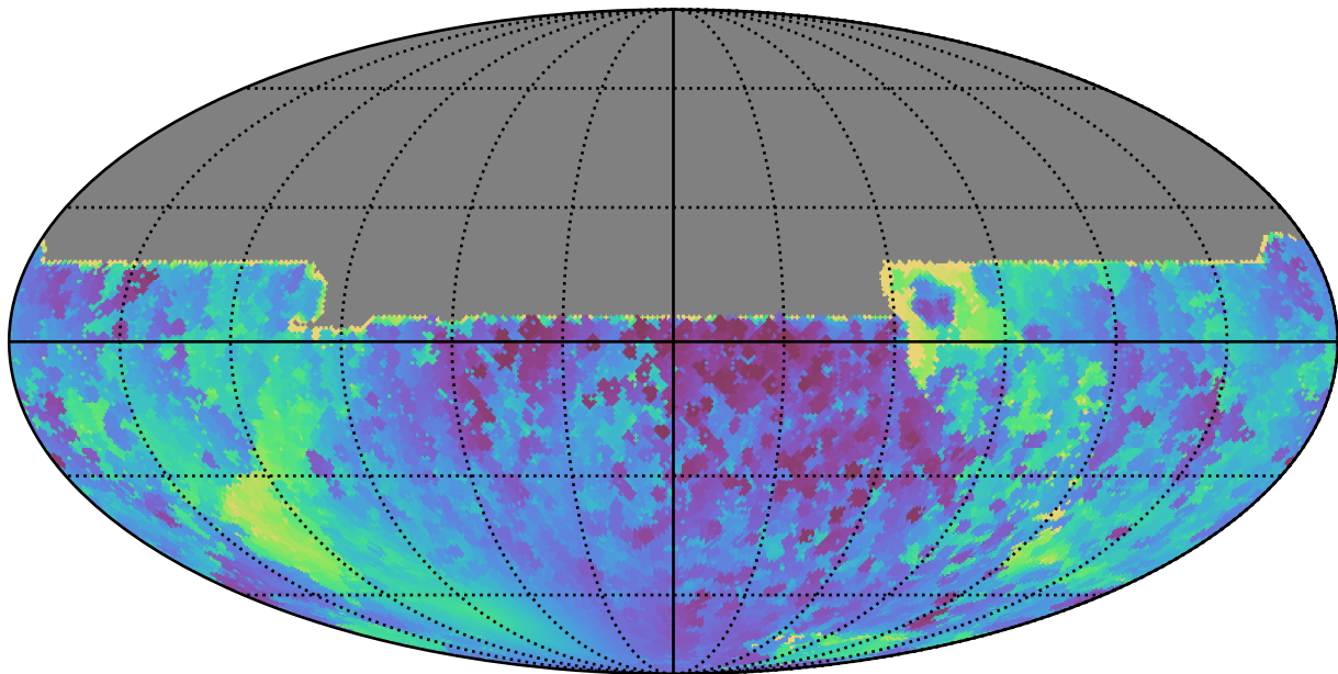
noroll_mjdp270_v3.4_10yrs All sky y band: Min solarElong
