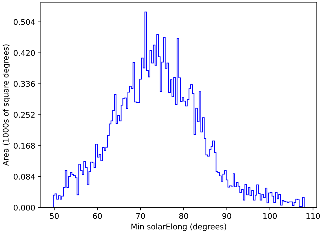
noroll_mjdp270_v3.4_10yrs All sky y band: Min solarElong
