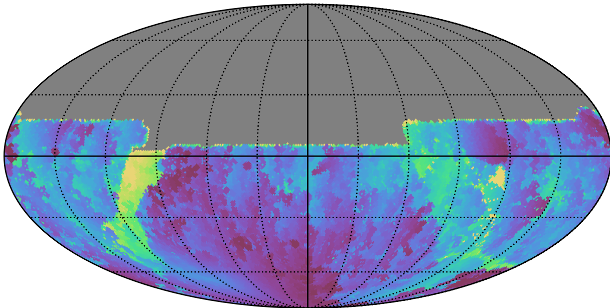
noroll_mjdp270_v3.4_10yrs All sky u band: Min solarElong
