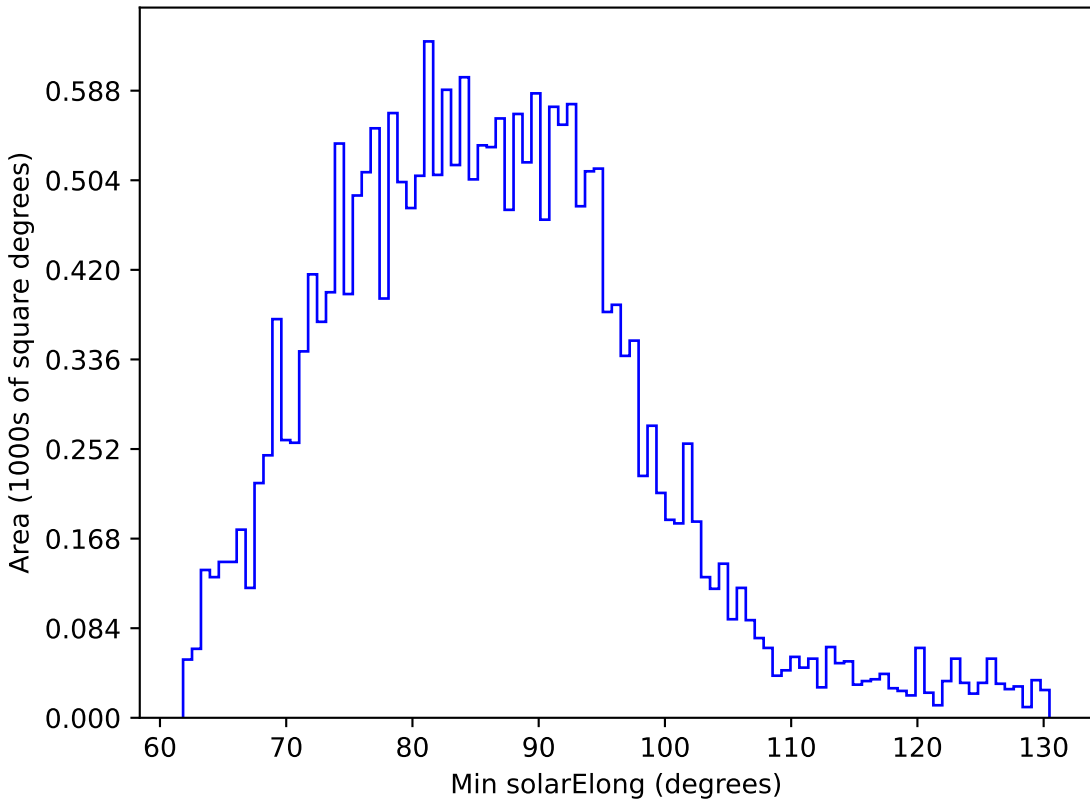
noroll_mjdp270_v3.4_10yrs All sky u band: Min solarElong
