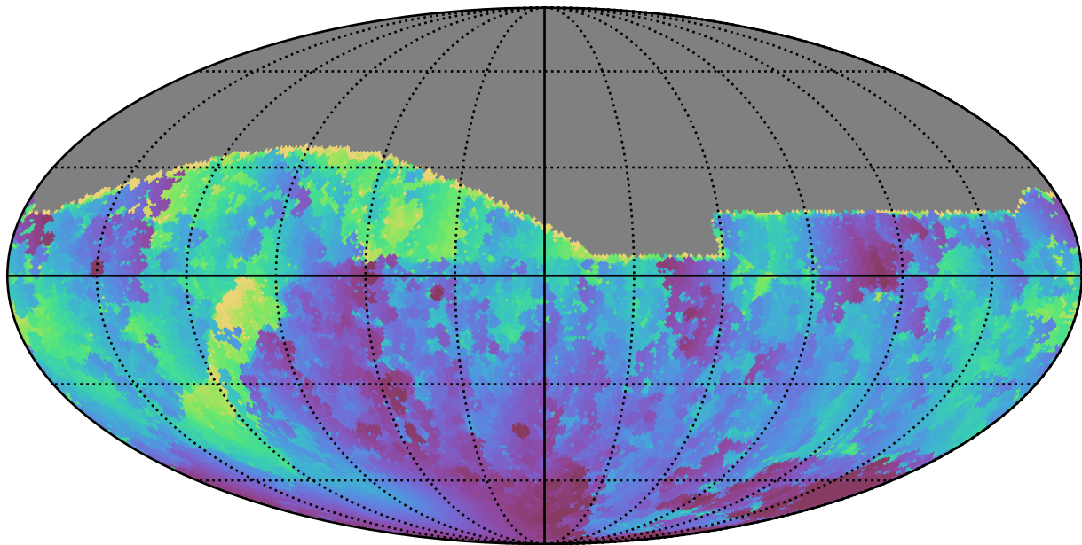
noroll_mjdp270_v3.4_10yrs All sky g band: Min solarElong
