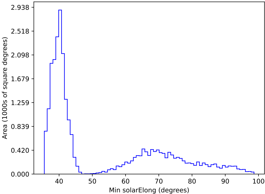
noroll_mjdp270_v3.4_10yrs All sky all bands: Min solarElong
