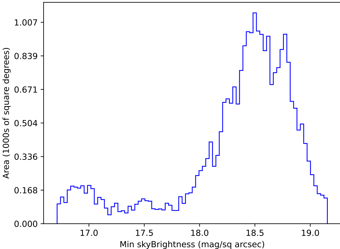
noroll_mjdp270_v3.4_10yrs Yr 1 z band: Min skyBrightness
