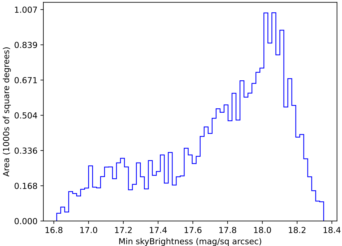
noroll_mjdp270_v3.4_10yrs Yr 1 y band: Min skyBrightness
