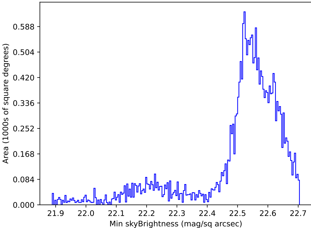
noroll_mjdp270_v3.4_10yrs Yr 1 u band: Min skyBrightness
