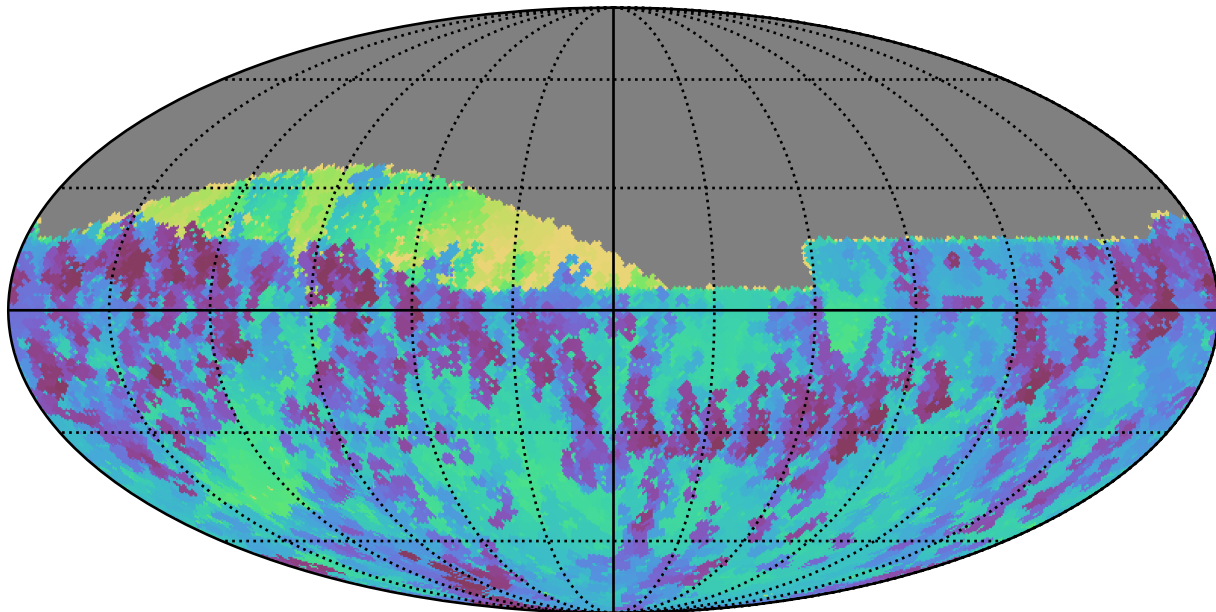
noroll_mjdp270_v3.4_10yrs Yr 1 all bands: Min skyBrightness
