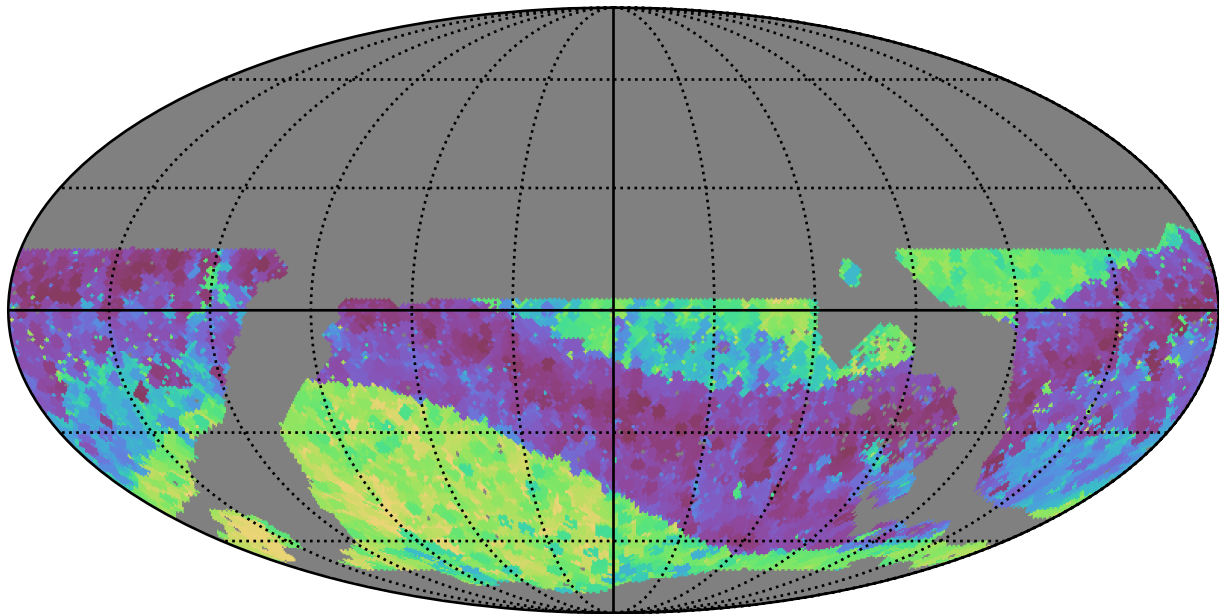
noroll_mjdp270_v3.4_10yrs WFD z band: Min skyBrightness
