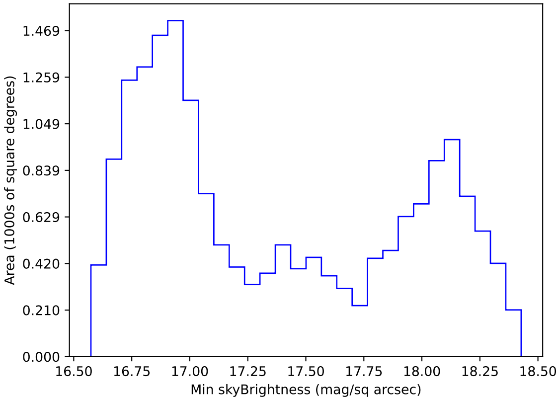
noroll_mjdp270_v3.4_10yrs WFD z band: Min skyBrightness
