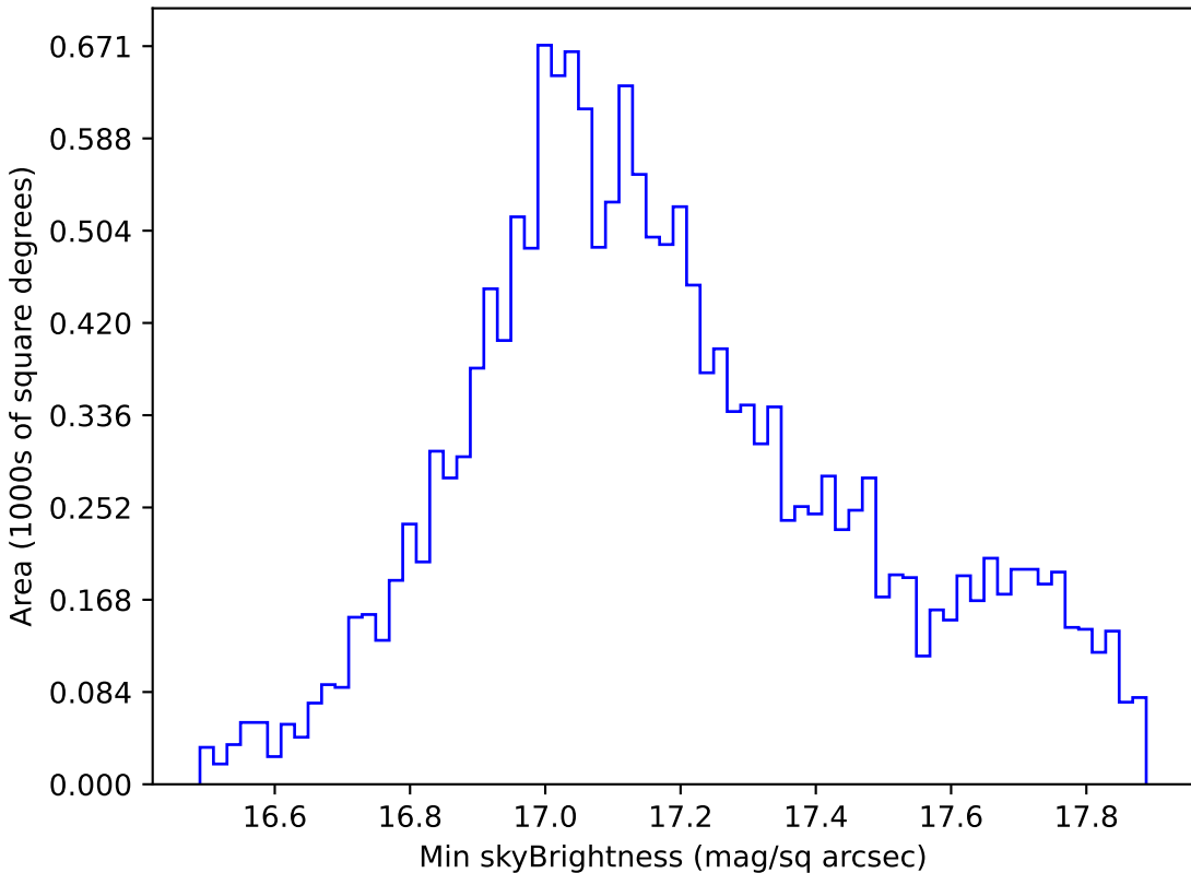
noroll_mjdp270_v3.4_10yrs WFD y band: Min skyBrightness
