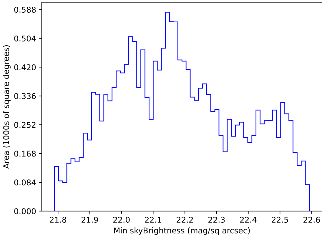
noroll_mjdp270_v3.4_10yrs WFD u band: Min skyBrightness
