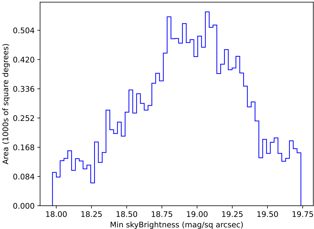
noroll_mjdp270_v3.4_10yrs WFD r band: Min skyBrightness
