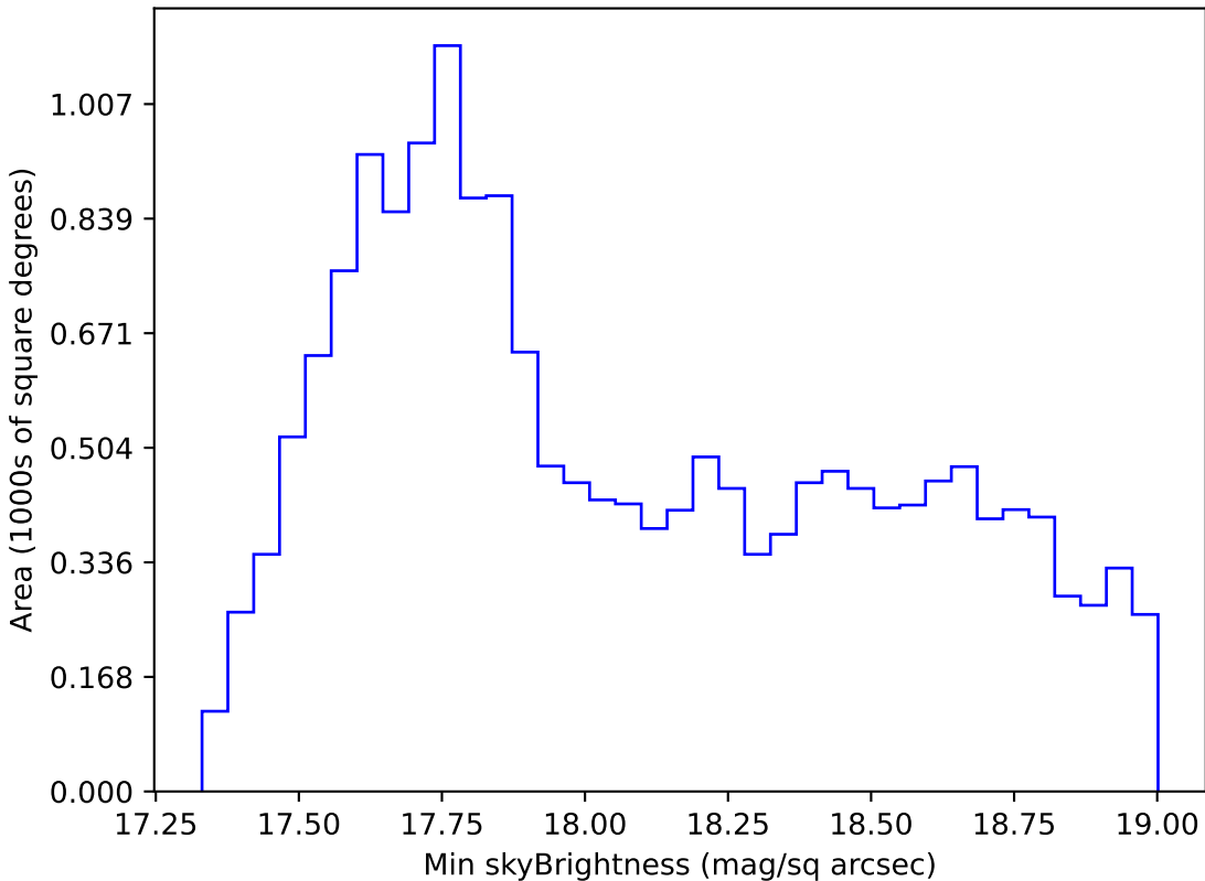
noroll_mjdp270_v3.4_10yrs WFD i band: Min skyBrightness
