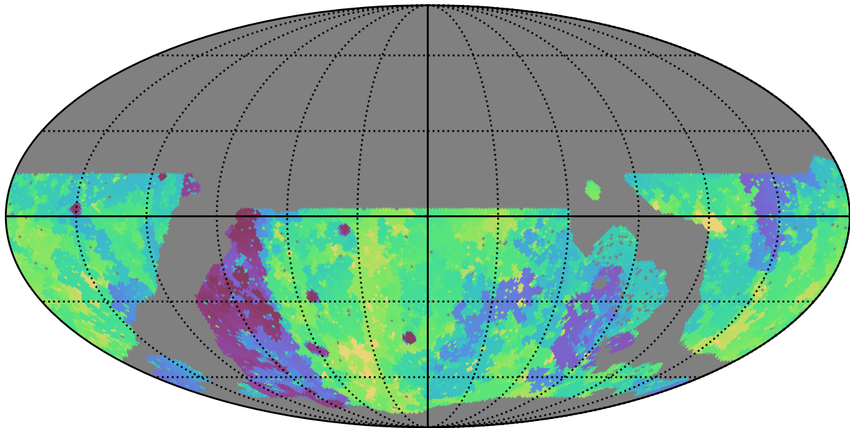
noroll_mjdp270_v3.4_10yrs WFD g band: Min skyBrightness
