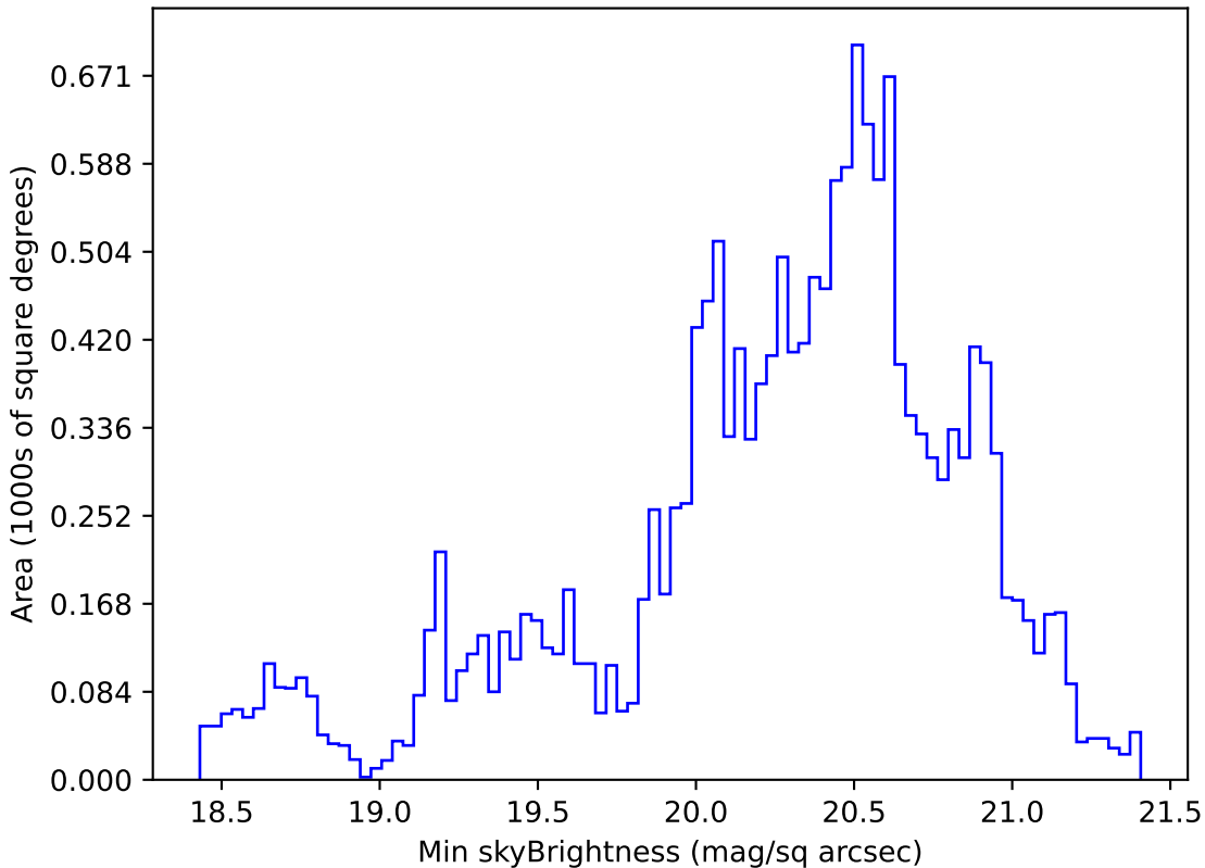
noroll_mjdp270_v3.4_10yrs WFD g band: Min skyBrightness
