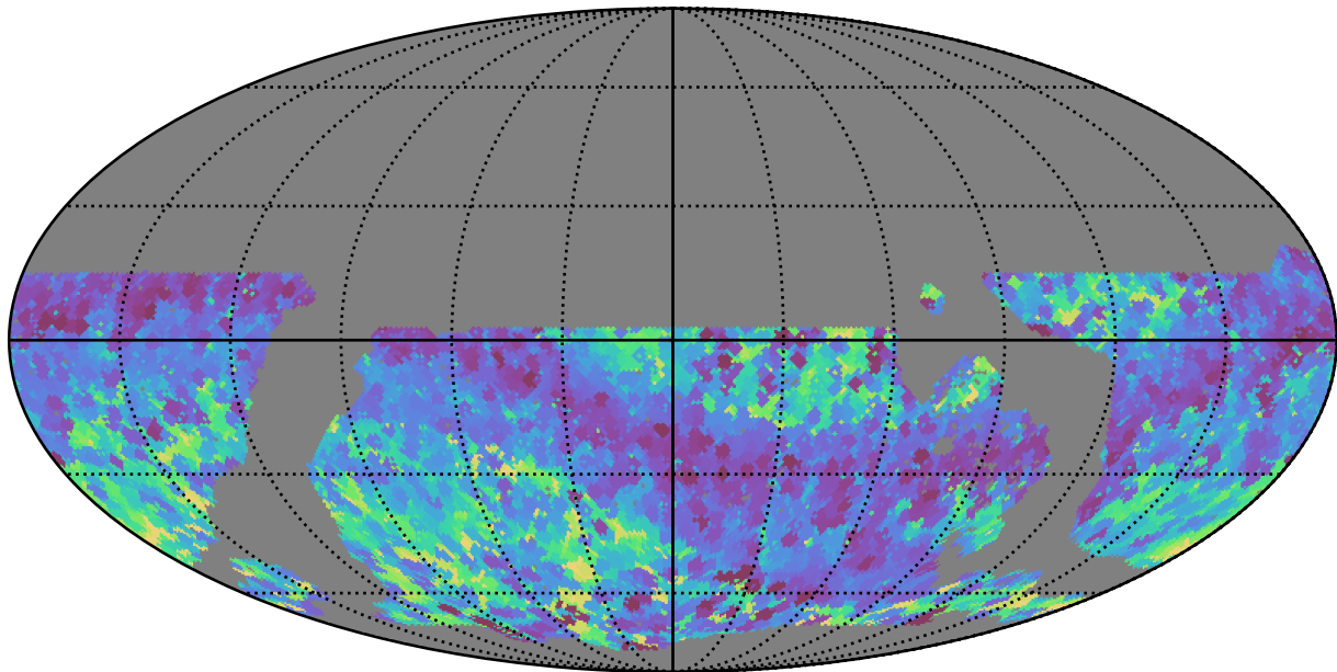
noroll_mjdp270_v3.4_10yrs WFD all bands: Min skyBrightness
