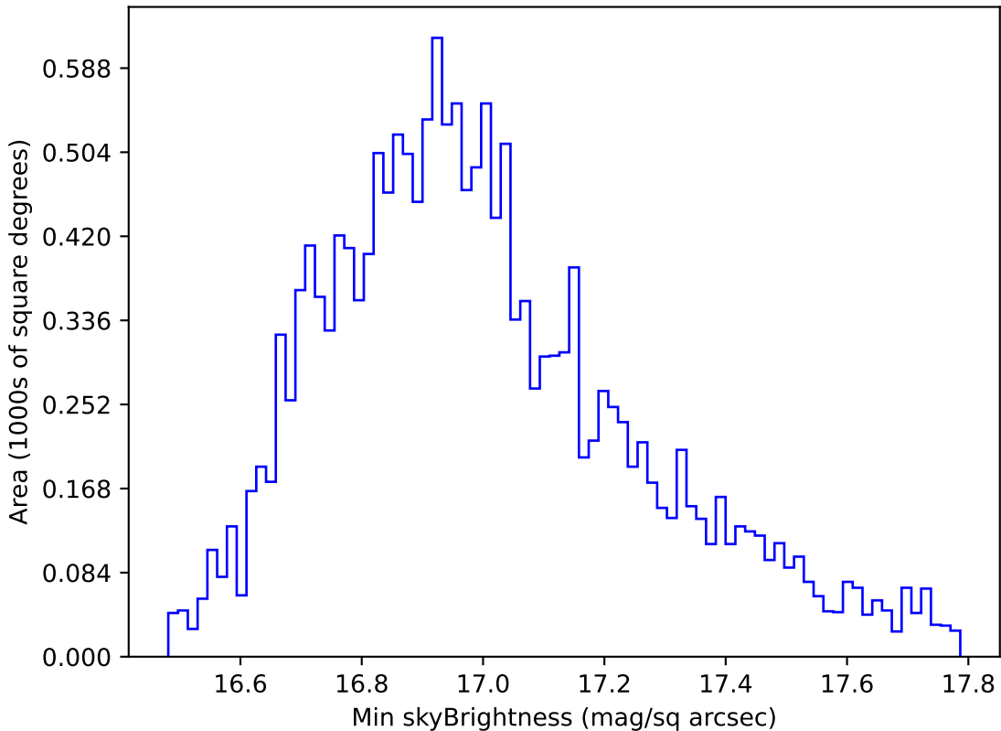
noroll_mjdp270_v3.4_10yrs WFD all bands: Min skyBrightness
