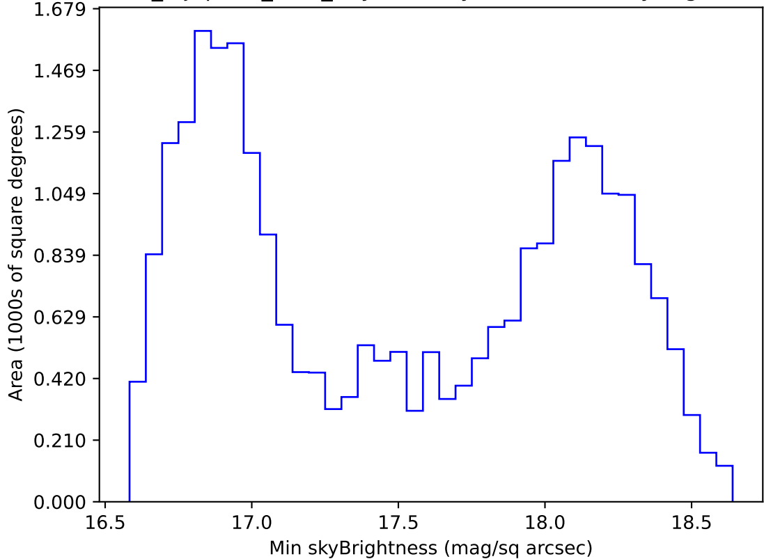
noroll_mjdp270_v3.4_10yrs All sky z band: Min skyBrightness
