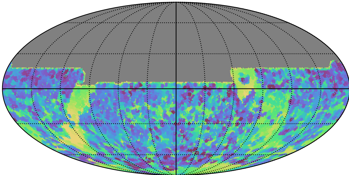
noroll_mjdp270_v3.4_10yrs All sky y band: Min skyBrightness
