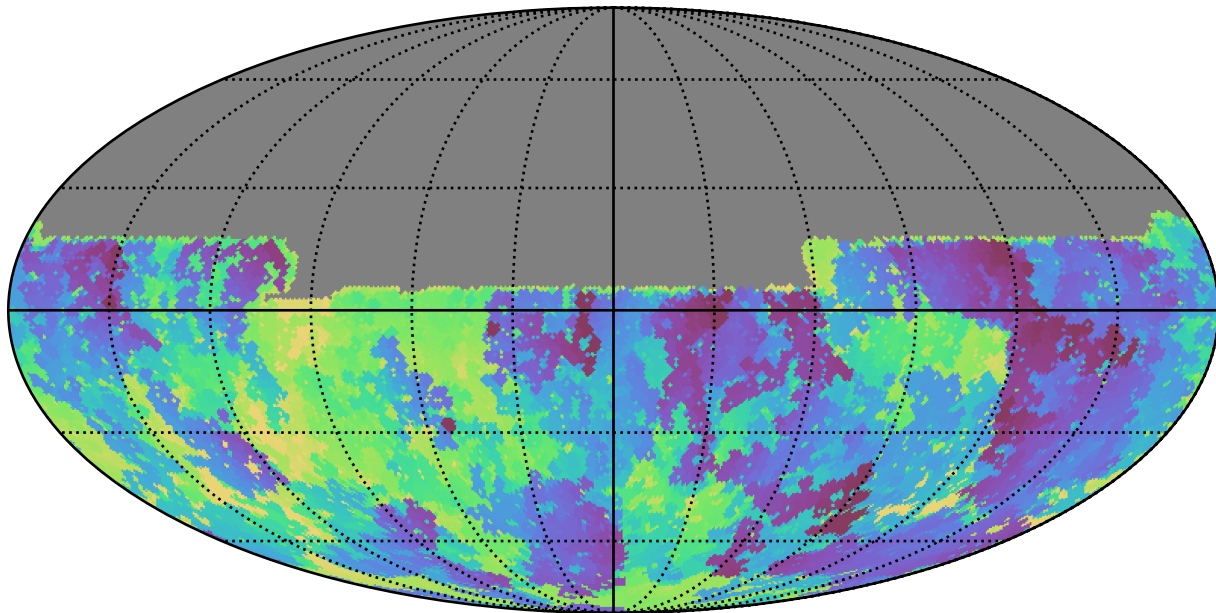
noroll_mjdp270_v3.4_10yrs All sky u band: Min skyBrightness
