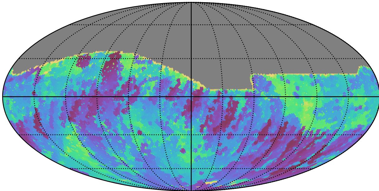
noroll_mjdp270_v3.4_10yrs All sky r band: Min skyBrightness
