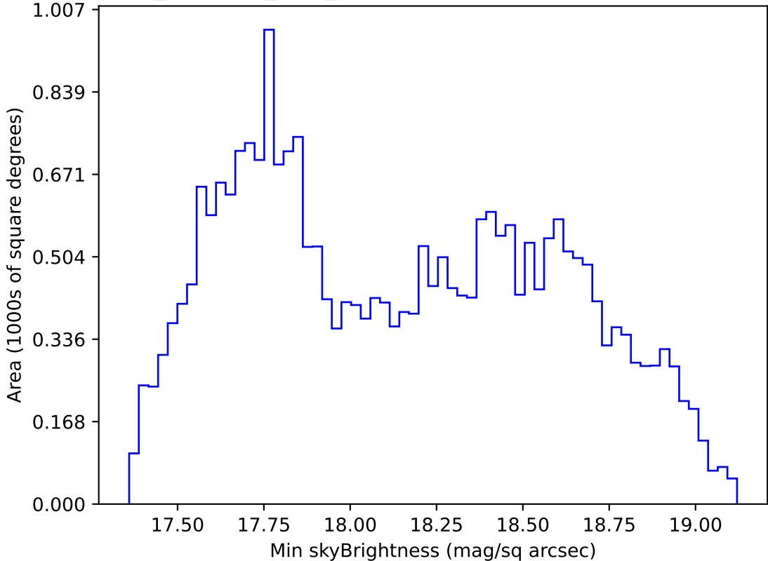
noroll_mjdp270_v3.4_10yrs All sky i band: Min skyBrightness
