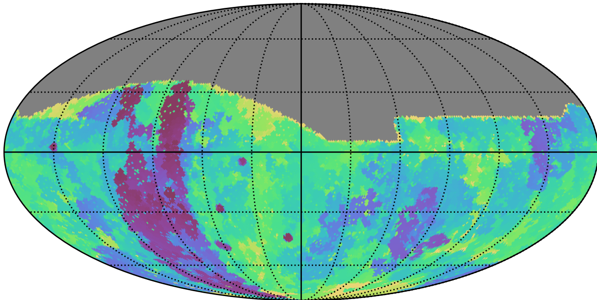
noroll_mjdp270_v3.4_10yrs All sky g band: Min skyBrightness
