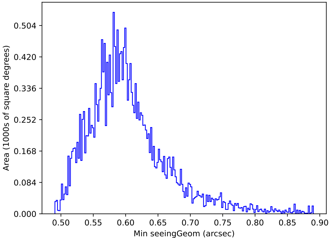
noroll_mjdp270_v3.4_10yrs Yr 1 y band: Min seeingGeom
