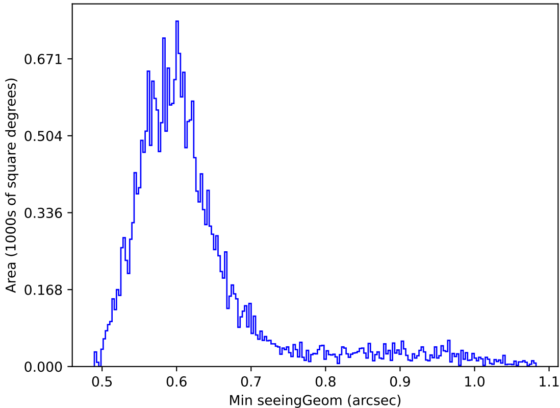
noroll_mjdp270_v3.4_10yrs Yr 1 r band: Min seeingGeom
