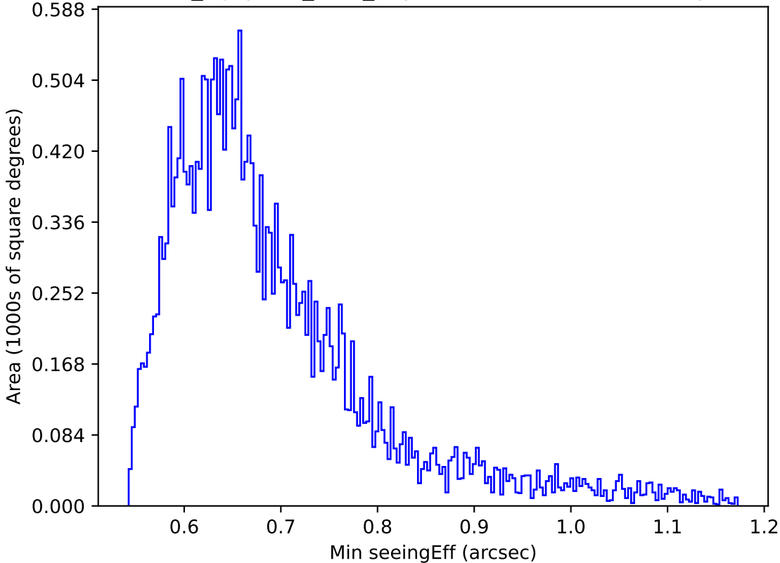
noroll_mjdp270_v3.4_10yrs Yr 1 z band: Min seeingEff
