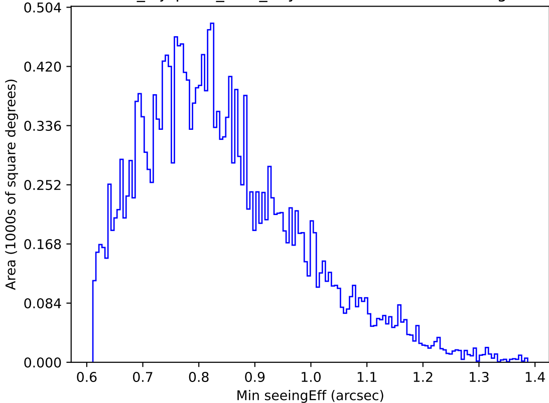
noroll_mjdp270_v3.4_10yrs Yr 1 u band: Min seeingEff
