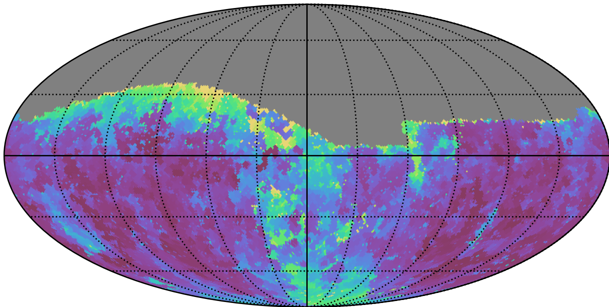
noroll_mjdp270_v3.4_10yrs Yr 1 g band: Min seeingEff
