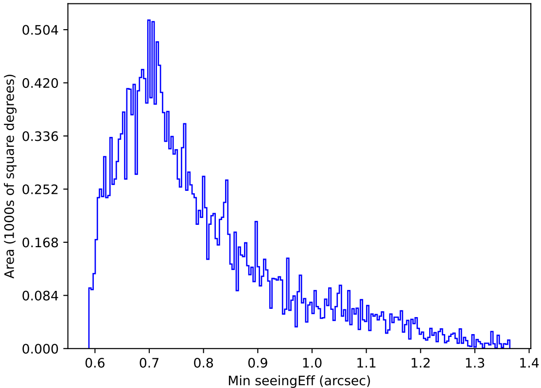
noroll_mjdp270_v3.4_10yrs Yr 1 g band: Min seeingEff
