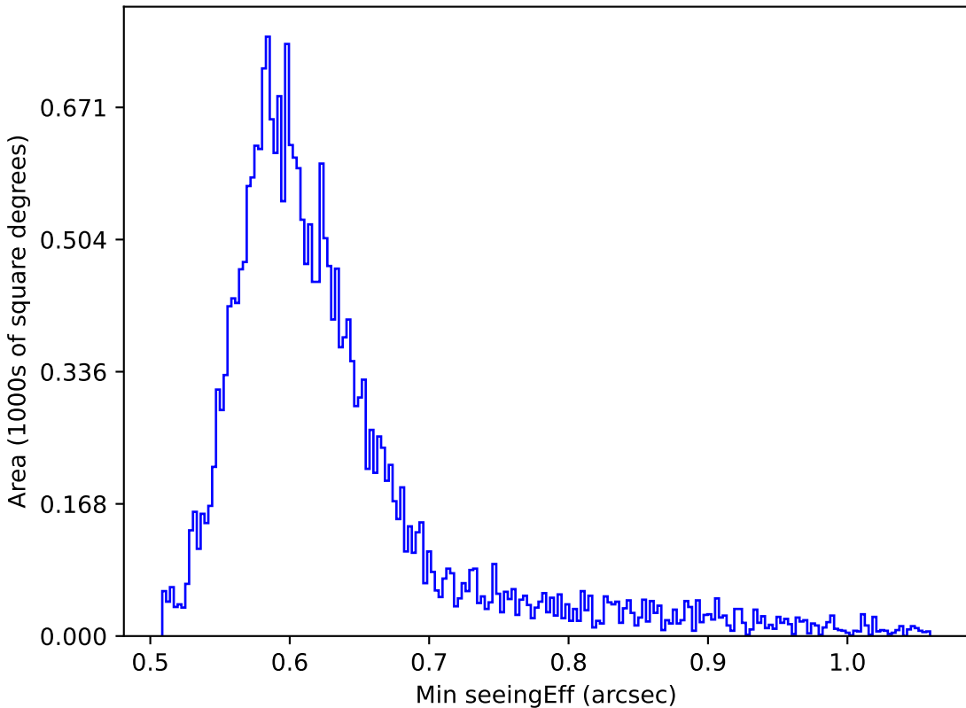
noroll_mjdp270_v3.4_10yrs Yr 1 all bands: Min seeingEff
