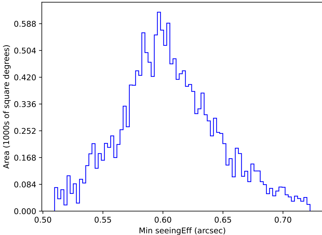
noroll_mjdp270_v3.4_10yrs WFD z band: Min seeingEff
