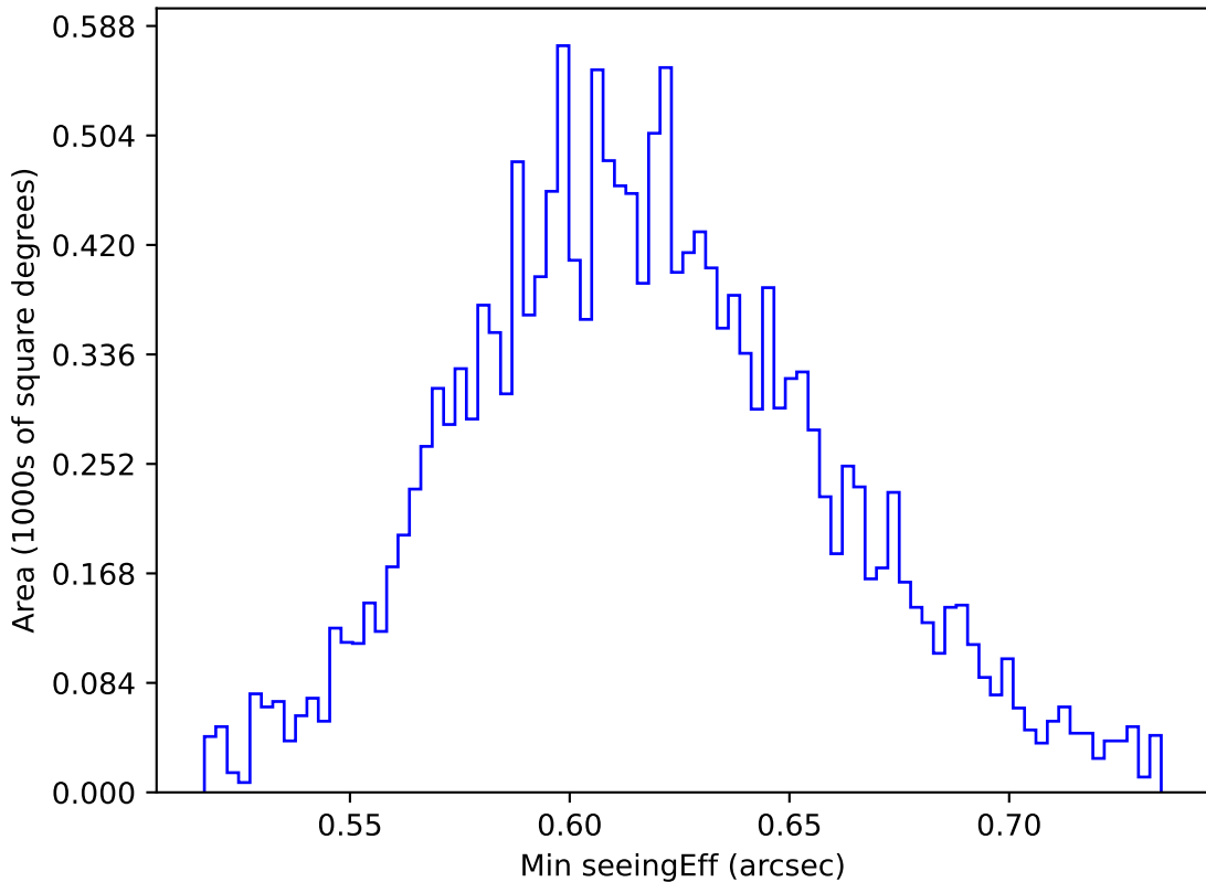
noroll_mjdp270_v3.4_10yrs WFD y band: Min seeingEff
