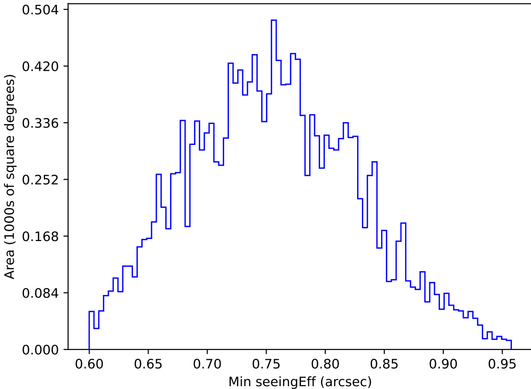
noroll_mjdp270_v3.4_10yrs WFD u band: Min seeingEff
