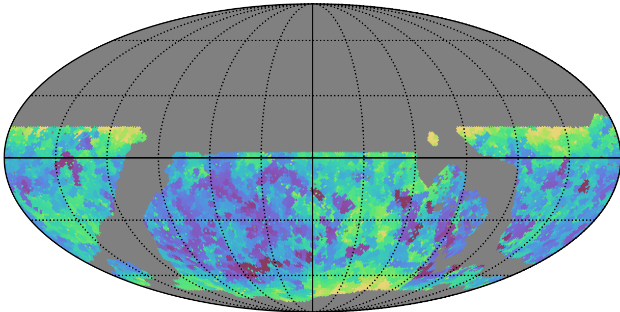
noroll_mjdp270_v3.4_10yrs WFD r band: Min seeingEff
