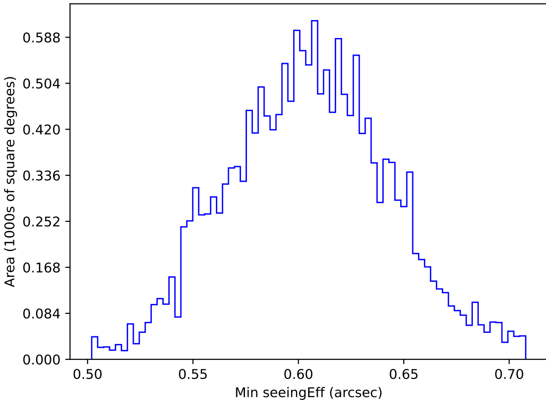
noroll_mjdp270_v3.4_10yrs WFD r band: Min seeingEff
