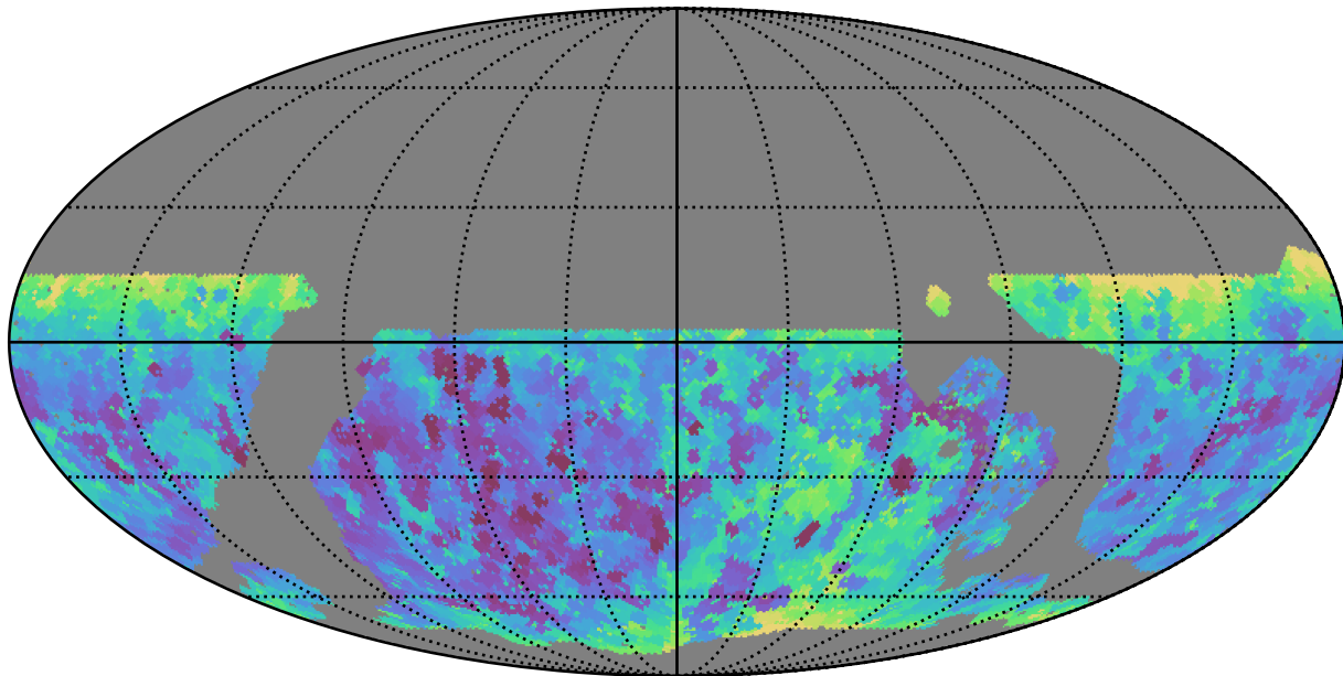
noroll_mjdp270_v3.4_10yrs WFD i band: Min seeingEff
