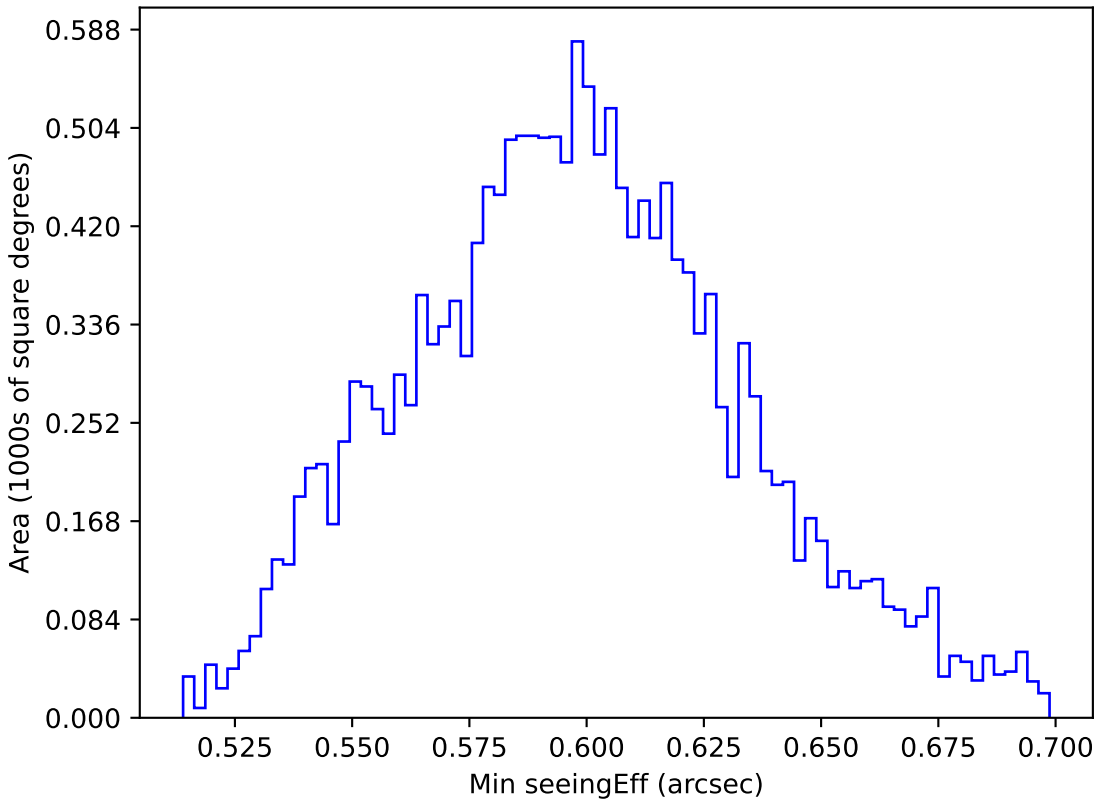
noroll_mjdp270_v3.4_10yrs WFD i band: Min seeingEff
