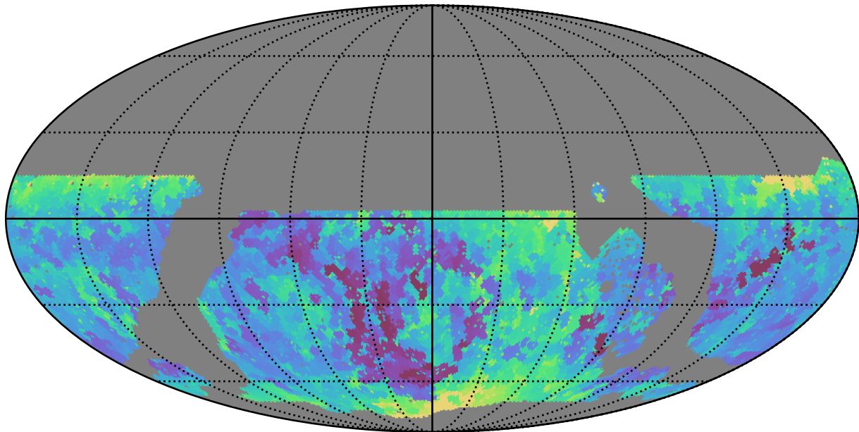
noroll_mjdp270_v3.4_10yrs WFD g band: Min seeingEff
