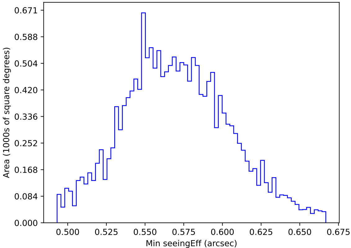
noroll_mjdp270_v3.4_10yrs WFD all bands: Min seeingEff
