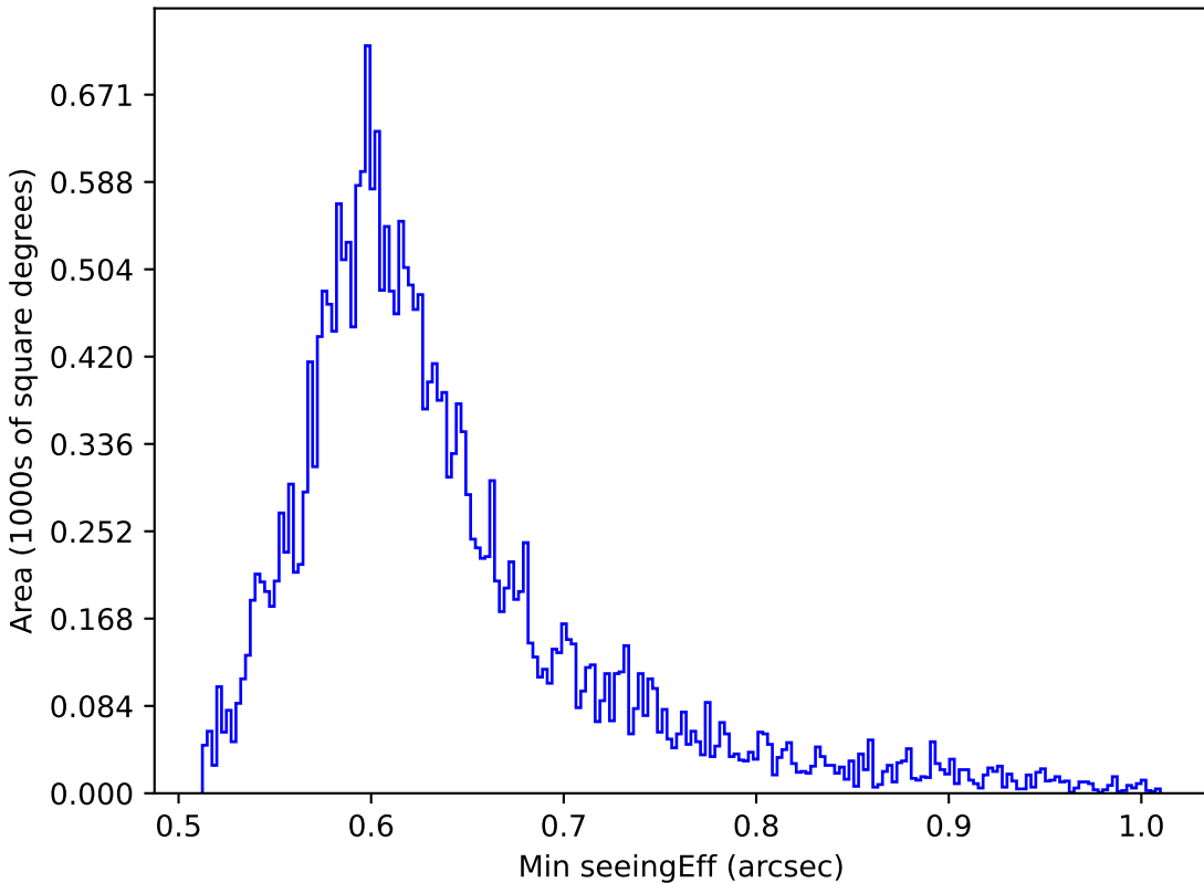
noroll_mjdp270_v3.4_10yrs All sky z band: Min seeingEff
