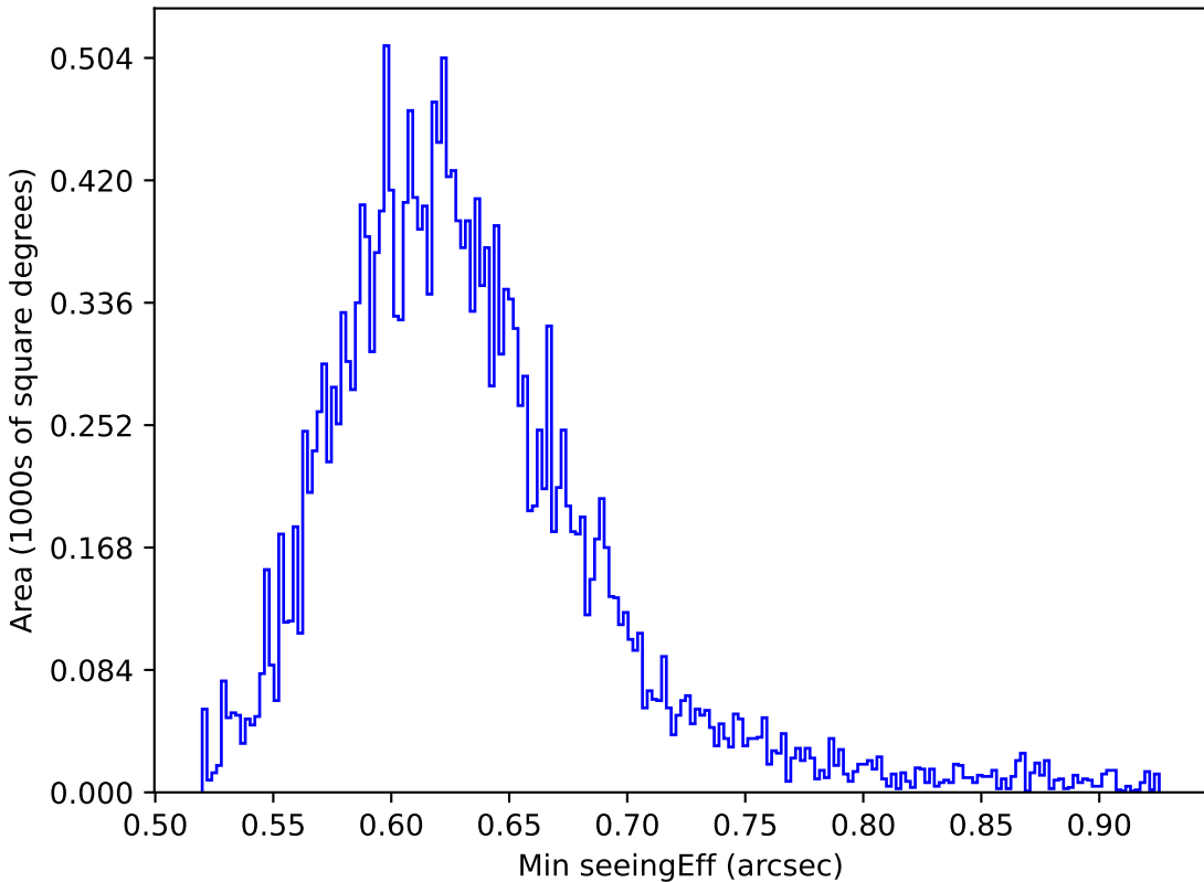
noroll_mjdp270_v3.4_10yrs All sky y band: Min seeingEff
