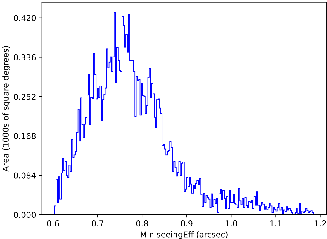
noroll_mjdp270_v3.4_10yrs All sky u band: Min seeingEff
