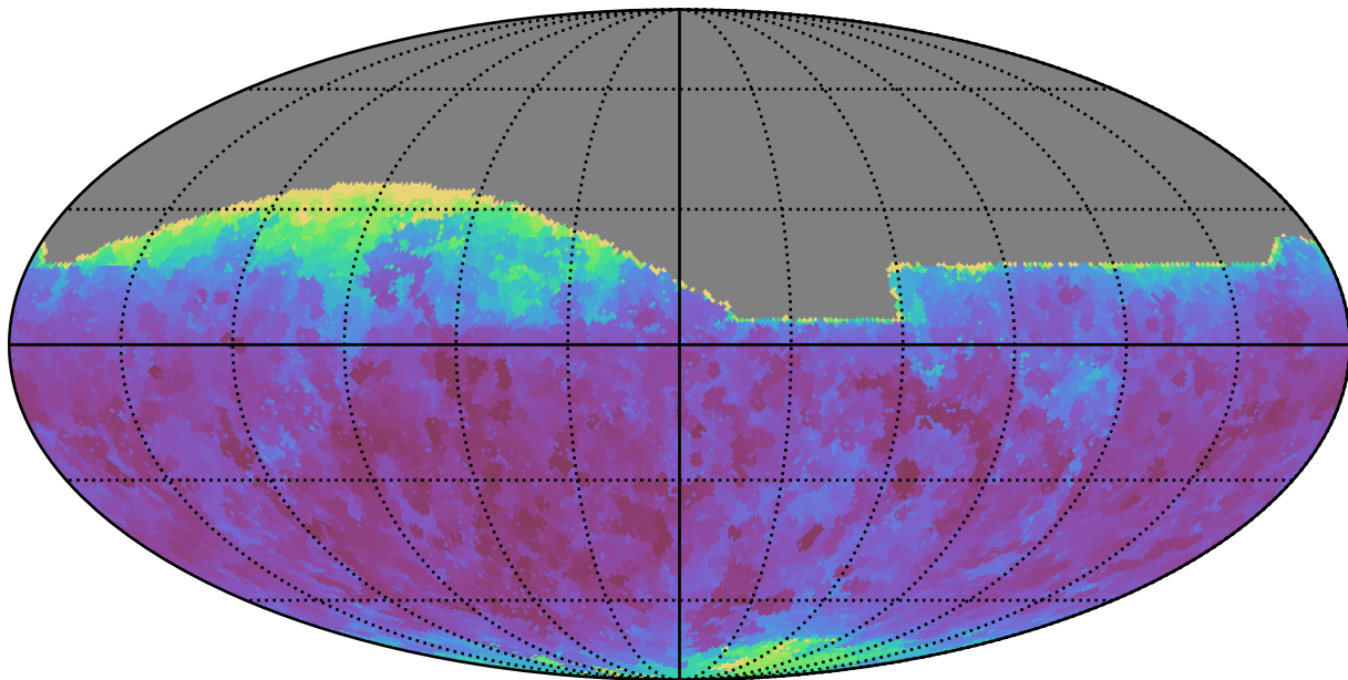
noroll_mjdp270_v3.4_10yrs All sky i band: Min seeingEff
