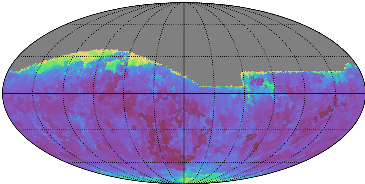
noroll_mjdp270_v3.4_10yrs All sky g band: Min seeingEff
