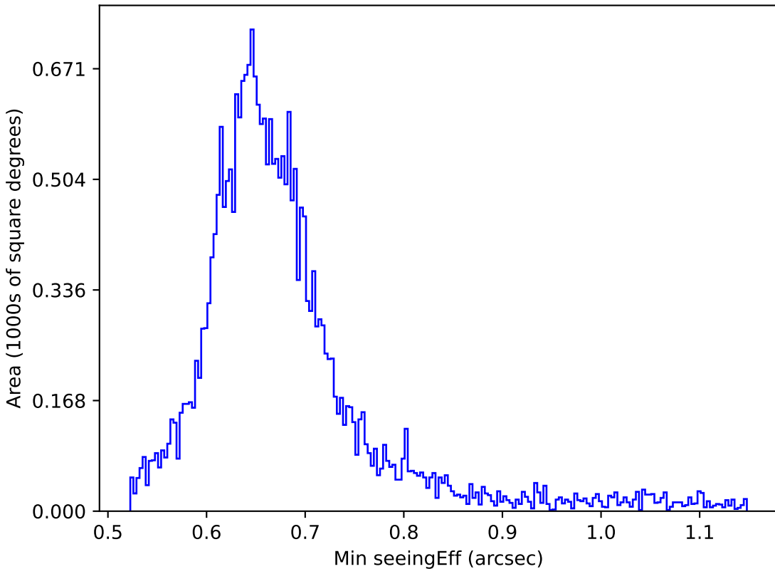
noroll_mjdp270_v3.4_10yrs All sky g band: Min seeingEff
